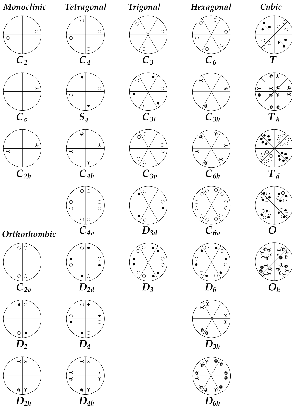
Figure 3.10. Stereograms for 30 point groups in 3D. The lines within the circles are visual aides, which in several cases correspond to reflection planes. The trigonal and hexagonal subsystems are shown separately, and the triclinic system (groups C_1 and C_i ) is not shown at all since it has trivial representations.
